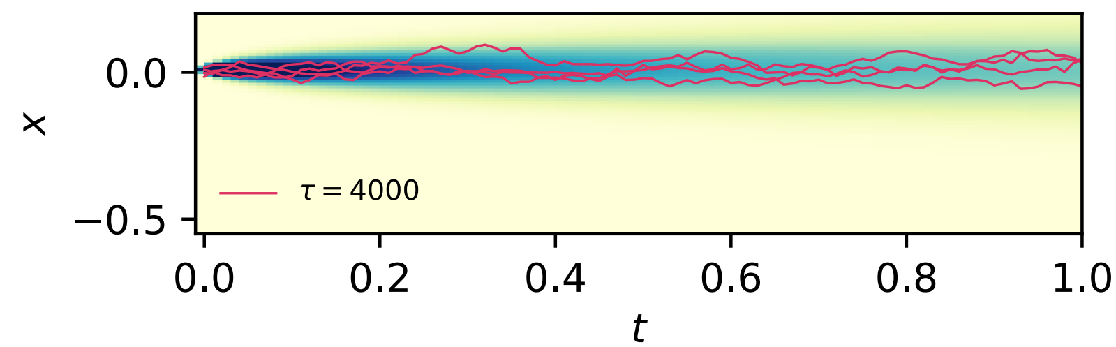
c) Sample paths, a final epoch
