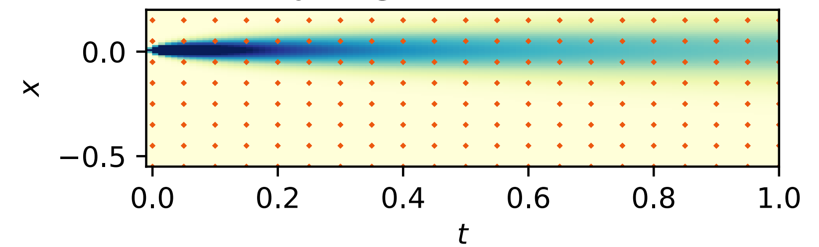
d) Uniform collocation points used by a grid-based solver
