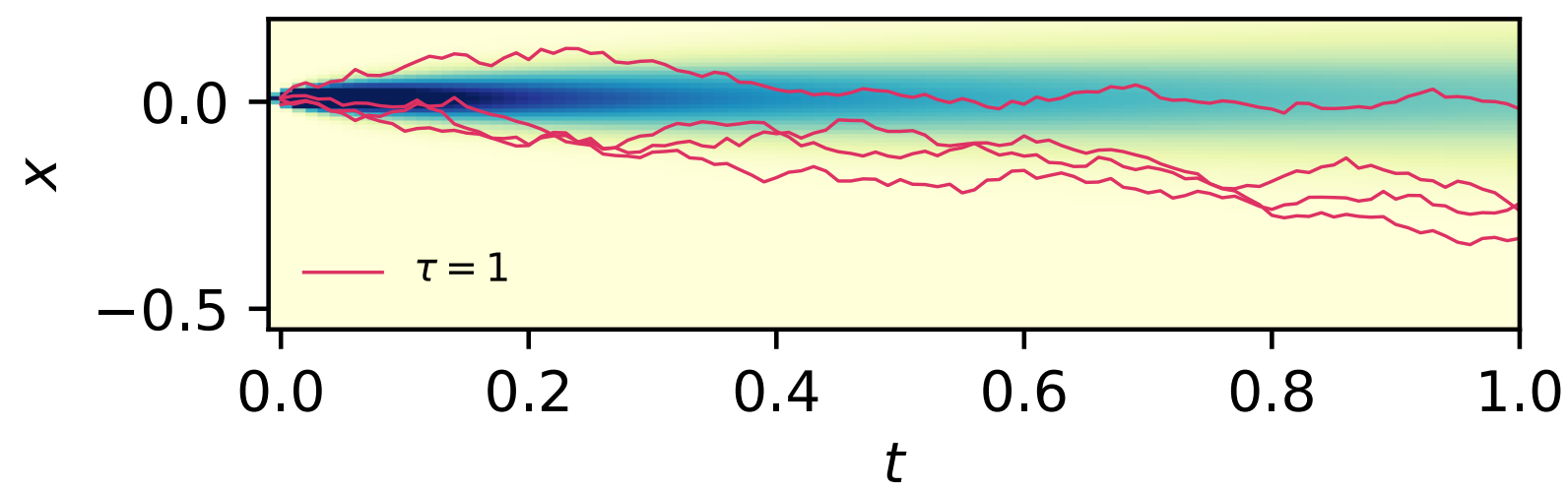
b) Sample paths, an early epoch
