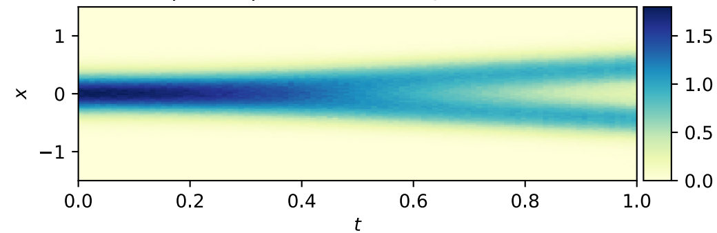
|\Psi(x_i, t)|^2, i = 1, 2 t-VMC prediction
