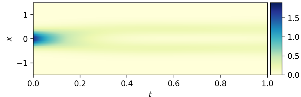
|\Psi(x_i, t)|^2, i = 1, 2 PINN prediction
