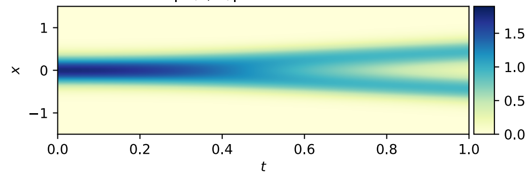
|\Psi(x_i, t)|^2, i = 1, 2 DSM prediction
